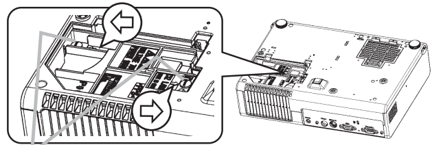
Screws marked by arrow
